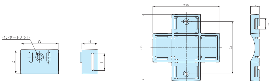
WPMB-M3・WPMB-M4
